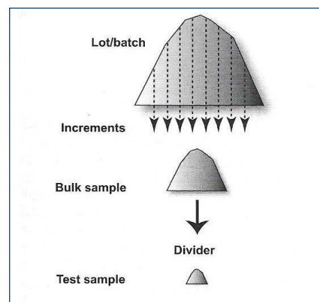
Figure 4: Test sample* (42)
